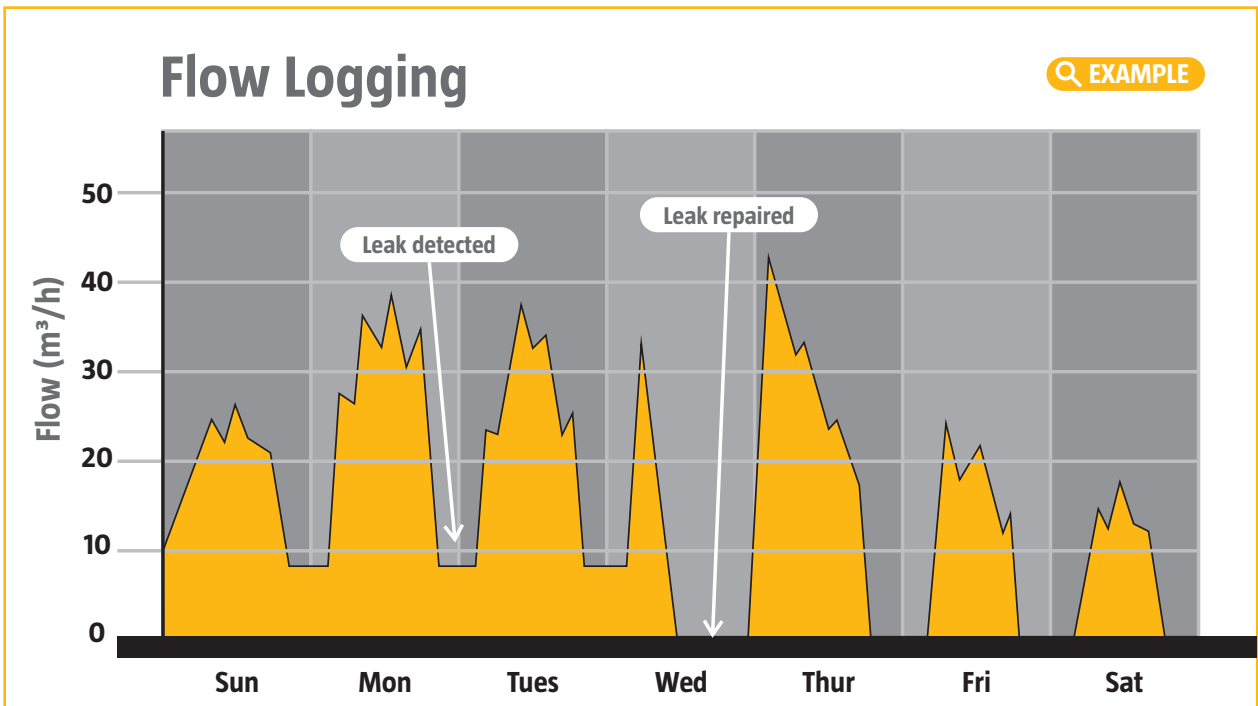
Early leak detection notification and monitoring of MNF (minimum night flow) from flow logging result.
